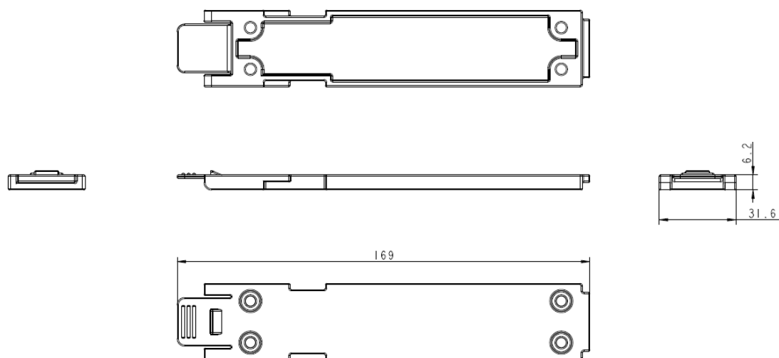
Figure 2 BA002 mounting bracket dimensions (mm)
