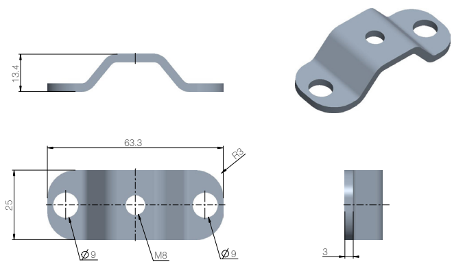
Figure 21 Bench foot
