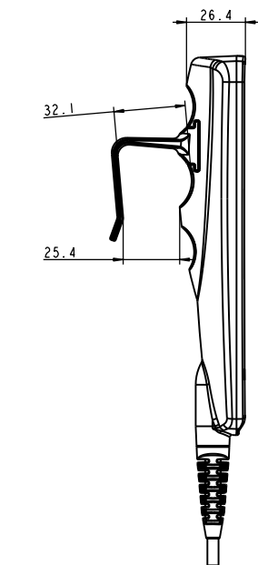
Hook option
