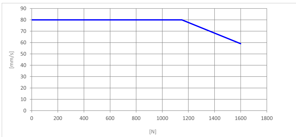
Figure 2 Two columns (equally loaded) - typical speed with CBD6S (230 V) 300 W
