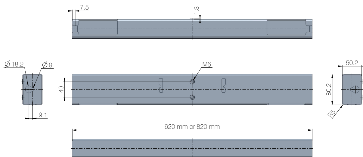
Figure 13 Cross member
