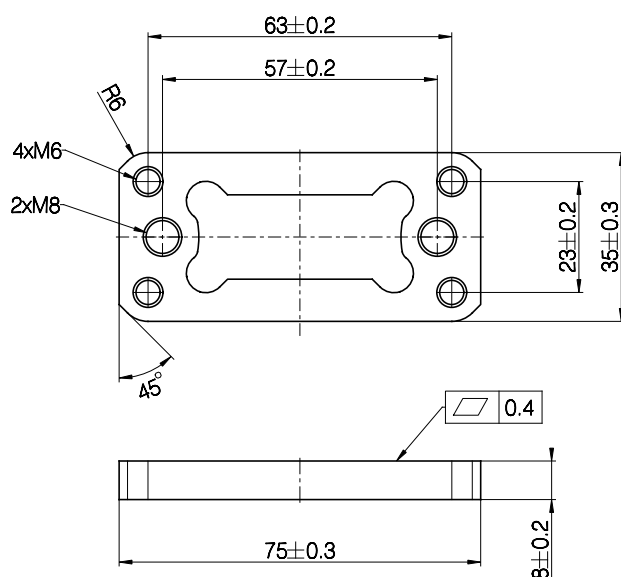
Figure 12 Bench bracket (types L and R)
