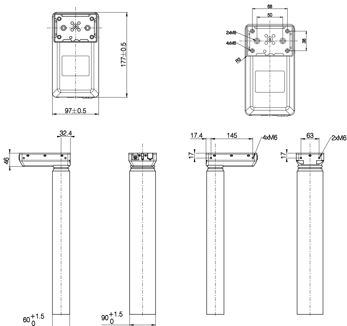
Figure 7 Built-in length, stroke length, and outer profile length
