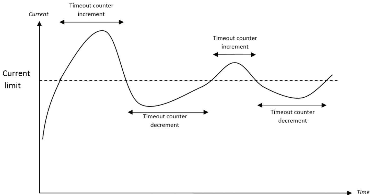
Figure 3. Dynamic current limit principle. When the Timeout counter max is reached, the actuator will stop and an over current error is triggered. The error is cleared when the actuator is activated in the opposite direction or by issuing a Clear error command.
