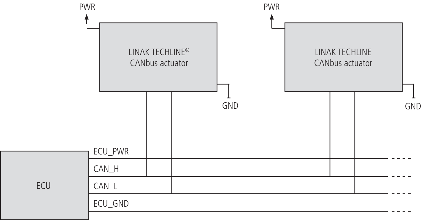
Figure 5. Power supply connection setup.
