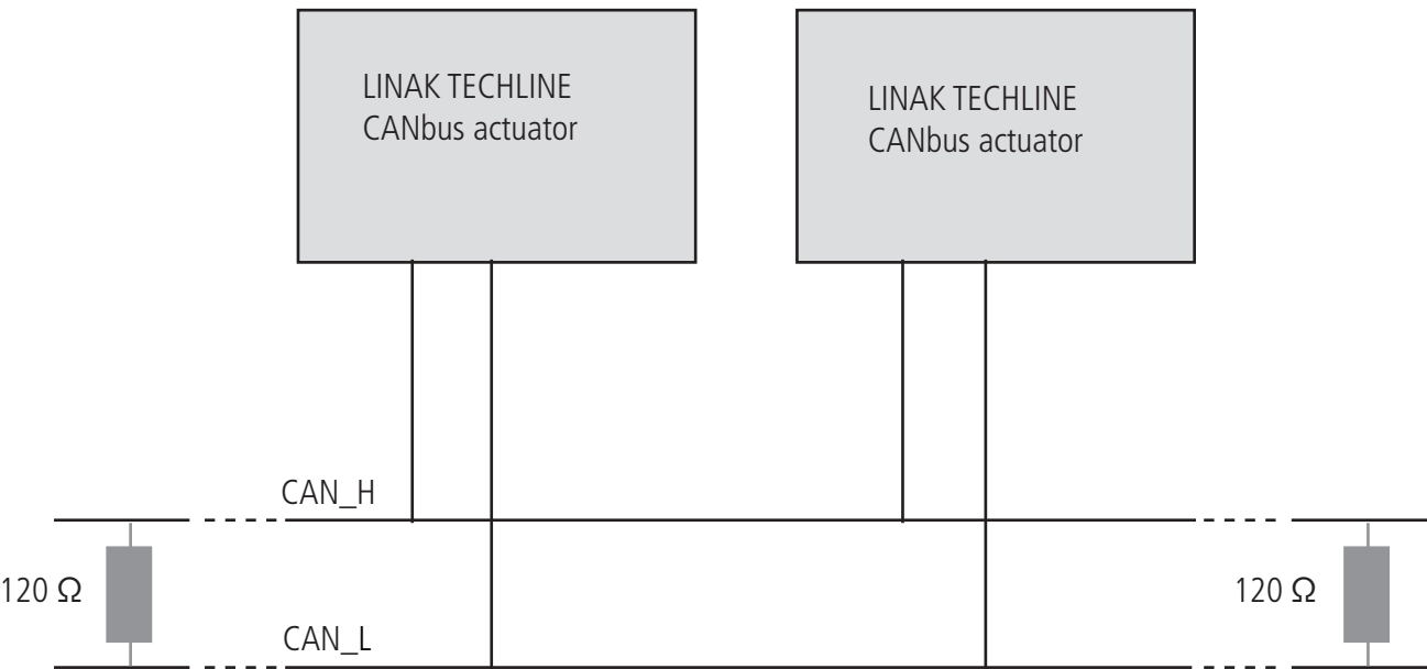
Figure 7. Termination connection diagram.
