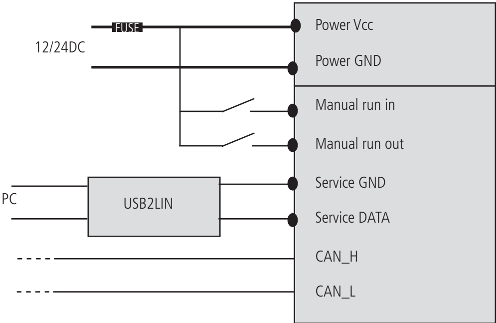
Figure 6. Connection pinout.
