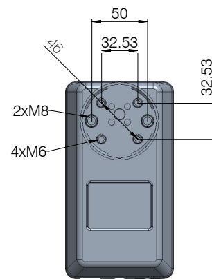
Bottom plate
