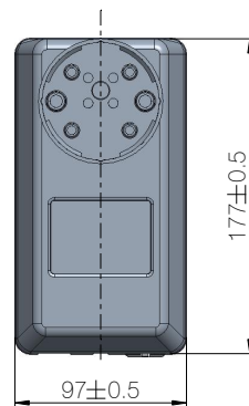
Motor housing
