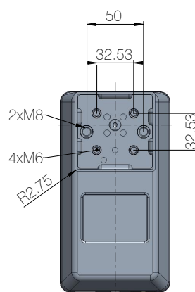
Bottom plate
