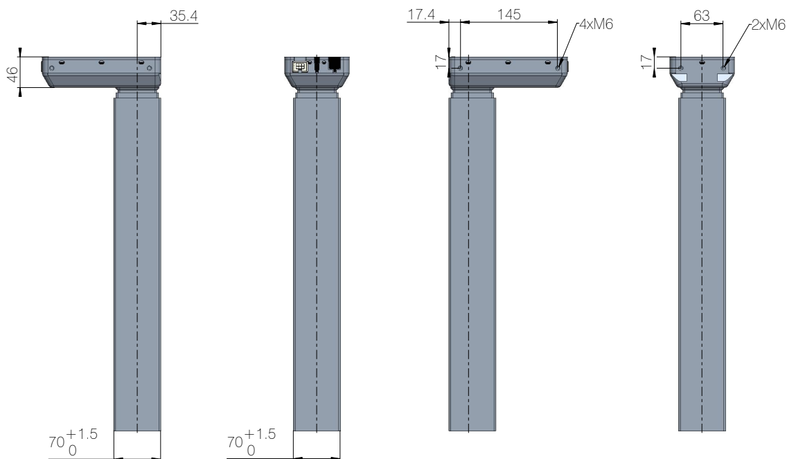
Profile dimensions (mm)
