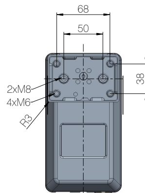
Bottom plate
