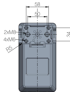
Bottom plate
