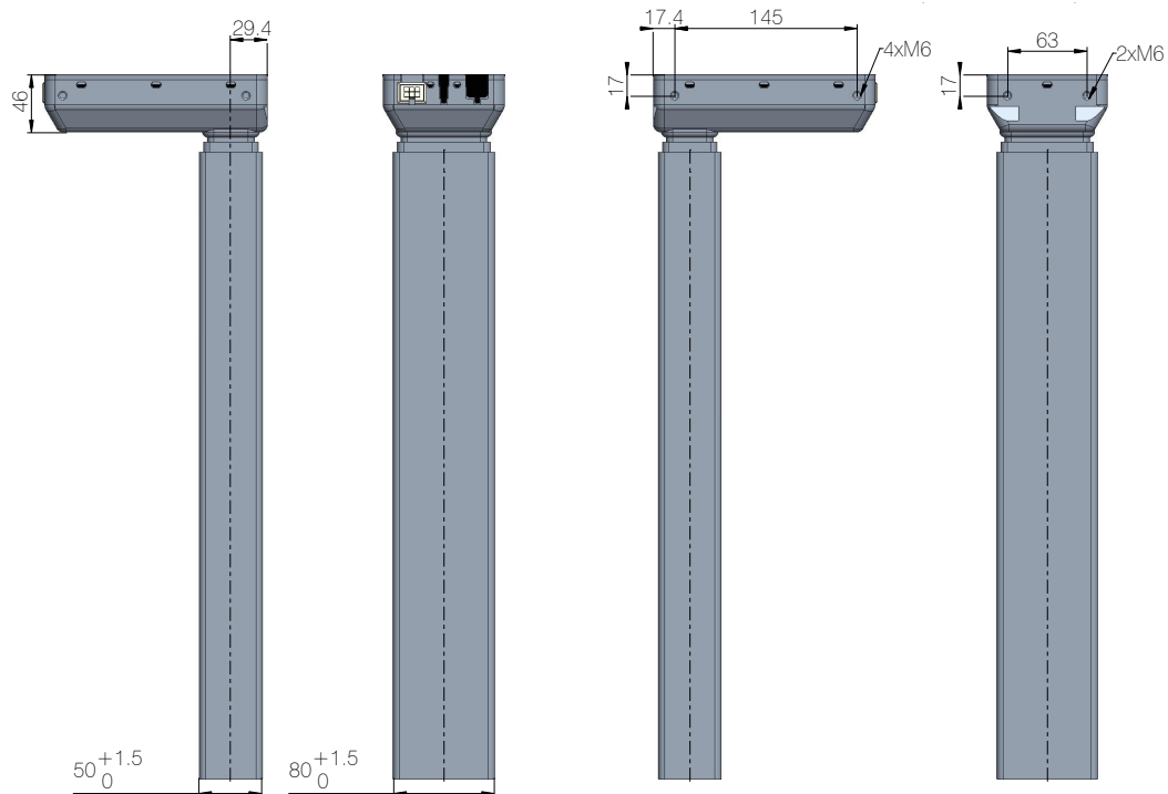
Profile dimensions (mm)
