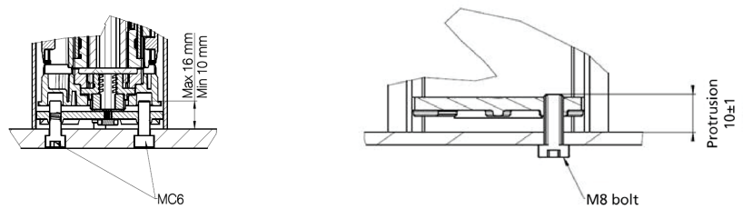
Figure 4 Column bottom mounted on desk foot (left: M6; right: M8)
