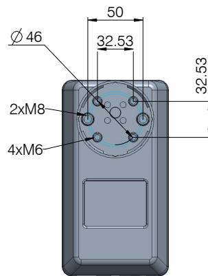
Figure 3 Bottom plate
