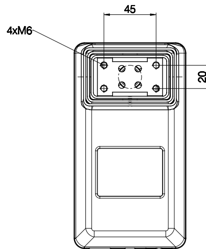
Figure 5 Bottom plate
