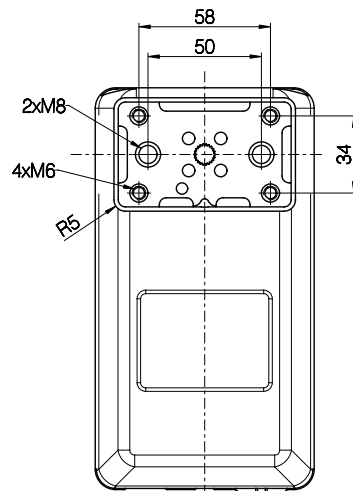
Figure 3 Bottom plate
