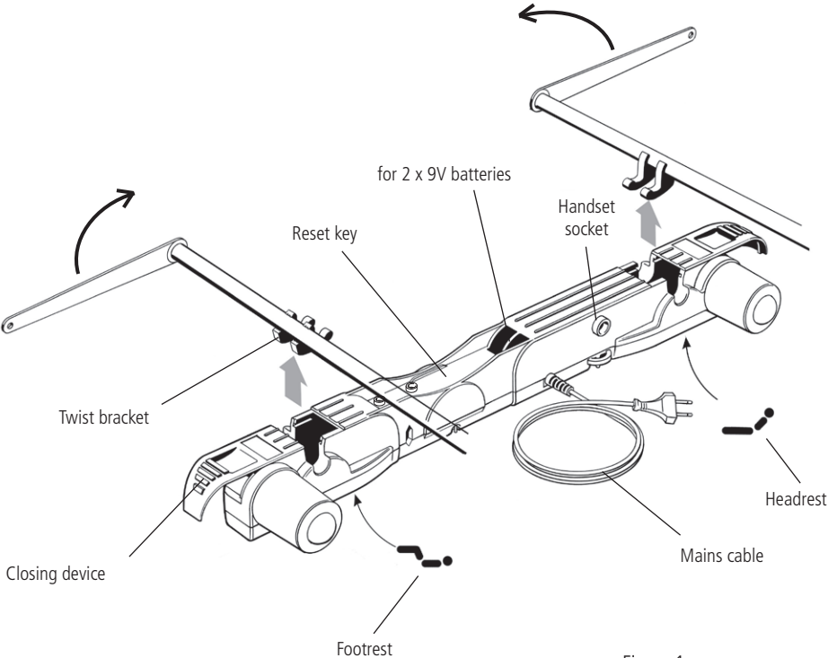
Figure 1 (Assembly overview) Connect the cable from the 2 x 9V batteries to the TD1 when connecting the mains.
